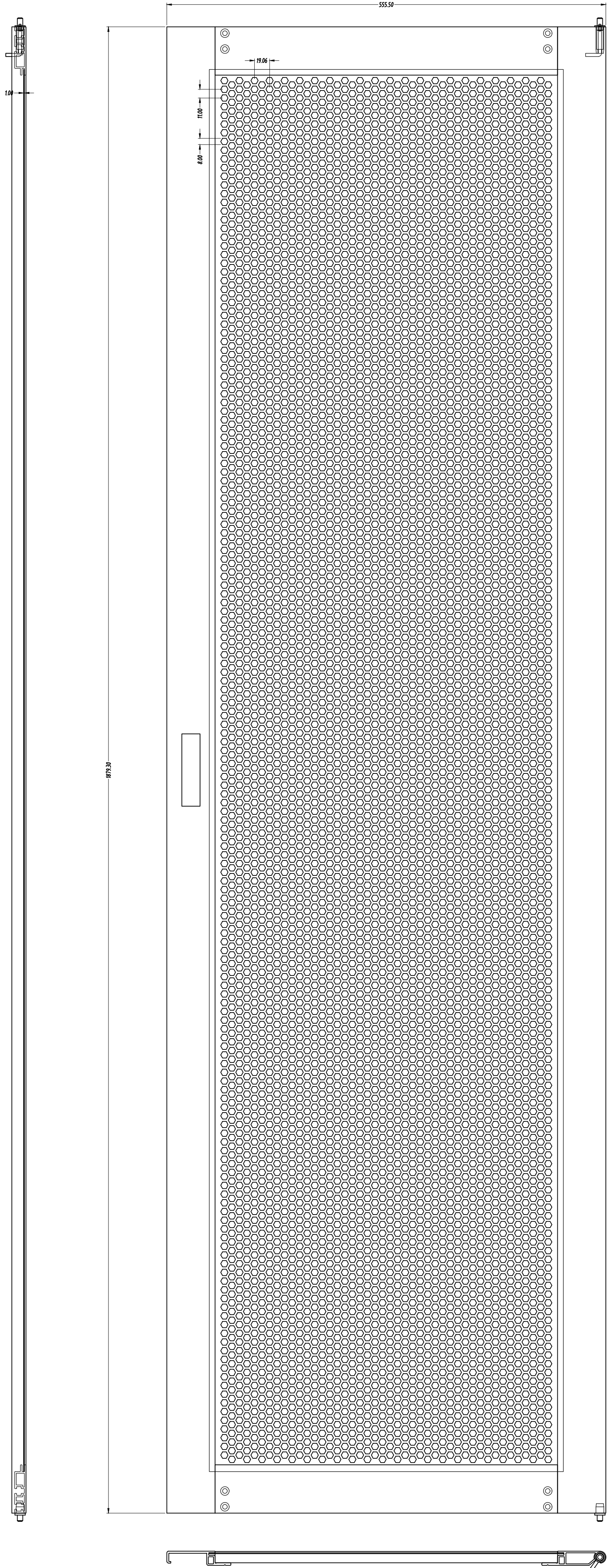
42U机柜后门尺寸: 1879.3*555.5*18mm
